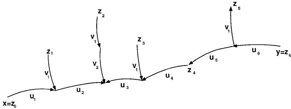
Figure 3. Case with s = 6, k = 3 .
